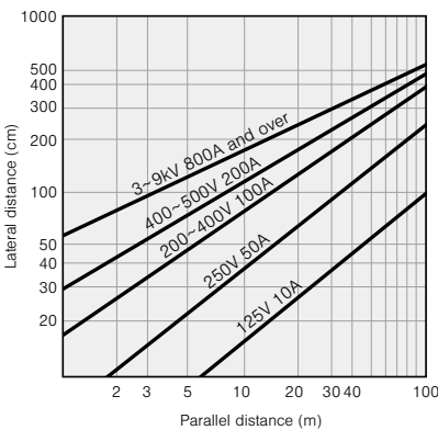
Fig. 4 Distances for positioning microphone and power cables when routing microphone cables via flexible metal conduit
