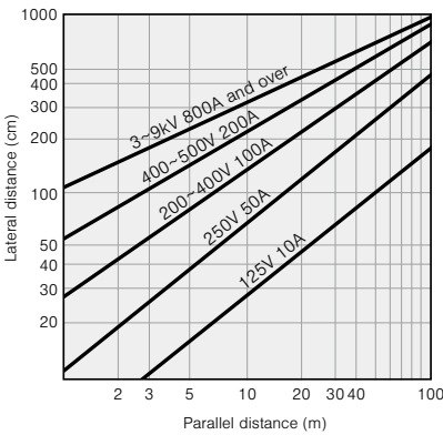
Fig. 3 Distances for positioning microphone and power cables
