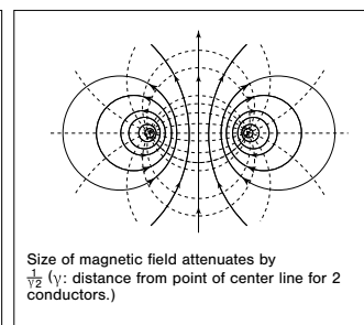
Two-conductor cable
